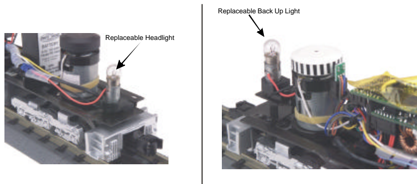
Figure 5: Removing The Replaceable Lights
