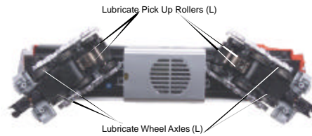
Figure 1. Lubrication Points on the Locomotive
