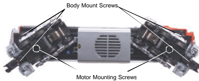
Figure 3: Body Removal Screw Locations
