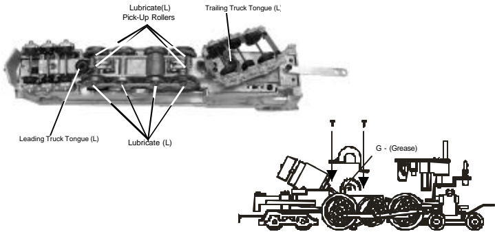
Figure 8: Lubricating The Locomotive Chassis
