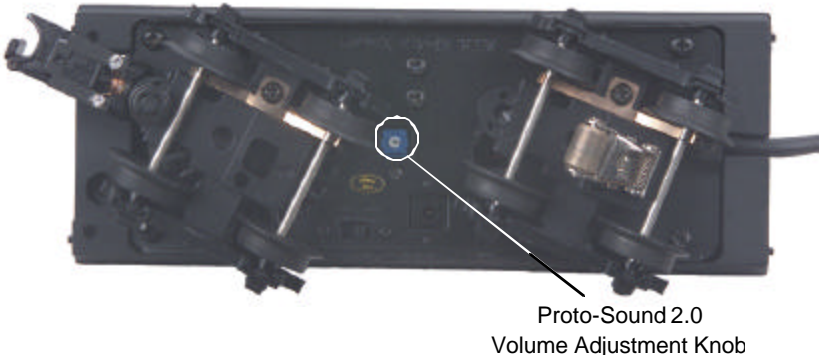
Figure 4: Manually Adjusting The Volume
