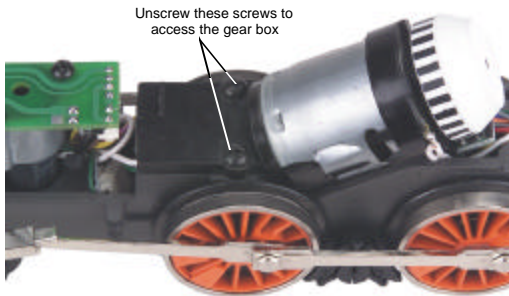
Figure 7: Motor Gearing Grease Plate Screws
