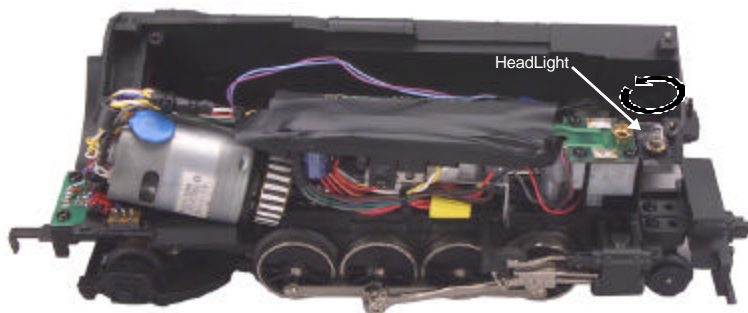
Figure 7. Replacing the Headlight
