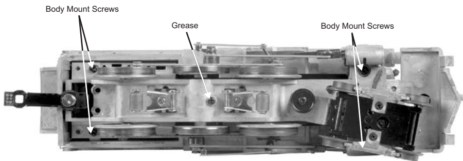
Figure 9: Body Mount Screws and Grease Points
