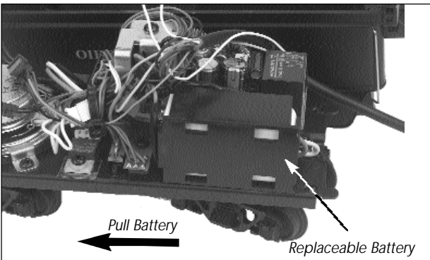
Figure 7- Replacing the Battery
