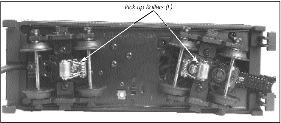
Figure 2b - Pick-up Rollers on the Tender
