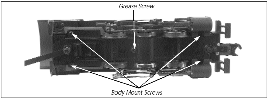
Figure 3 - Greasing points on the engine & location of body mount screws
