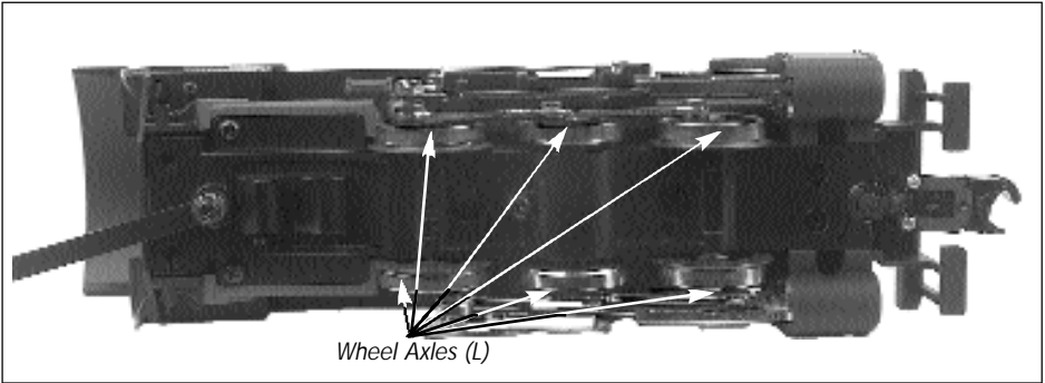
Figure 2a - Lubrication Points on the Engine
