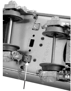
Manual Volume Control (4-6-2 Forty-Niner and 4-6-2 Torpedo)
