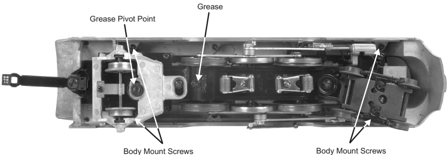
Figure: Body Mount Screws and Grease Points
