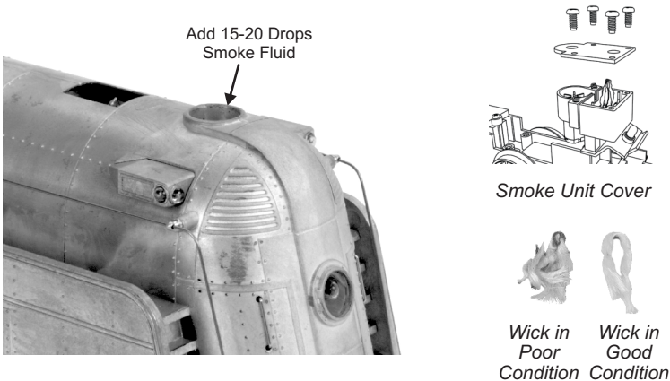
Figure: Adding Fluid
