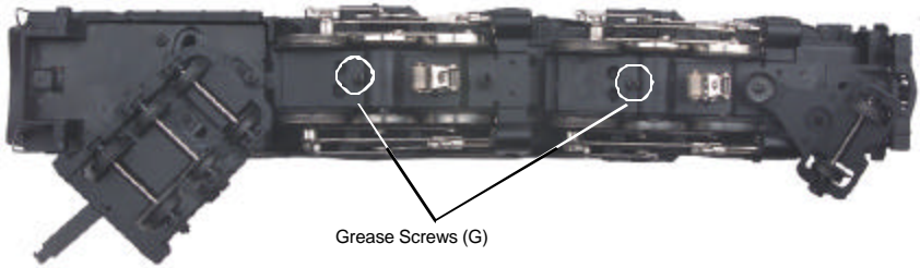
Figure 7: Motor Gearing Grease Plate Screws
