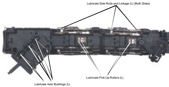
Figure 1. Lubrication Points on the Locomotive
