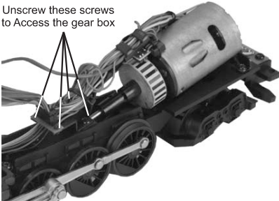
Figure 10: Motor Gearing Grease Plate Screws
