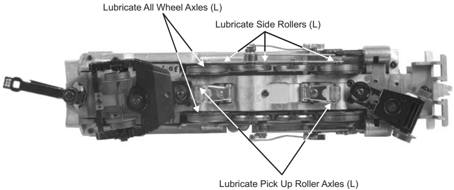
Figure 8: Lubricating the Locomotive
