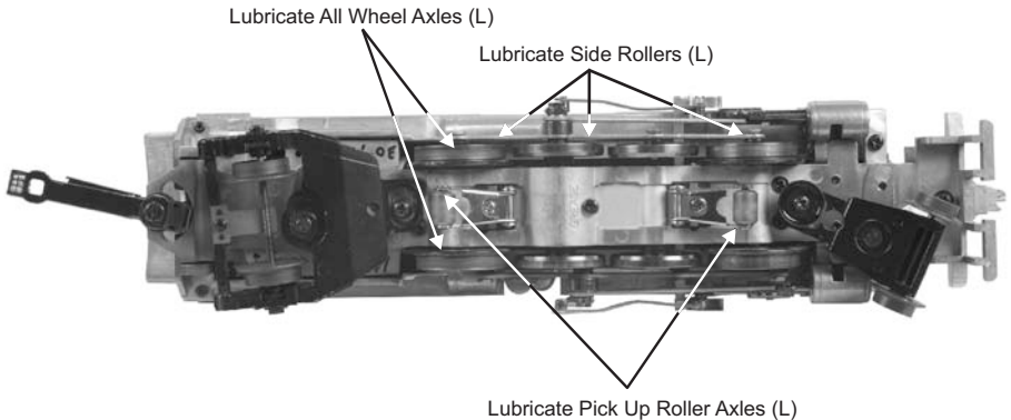
Fig. 1: Lubricating the Locomotive
