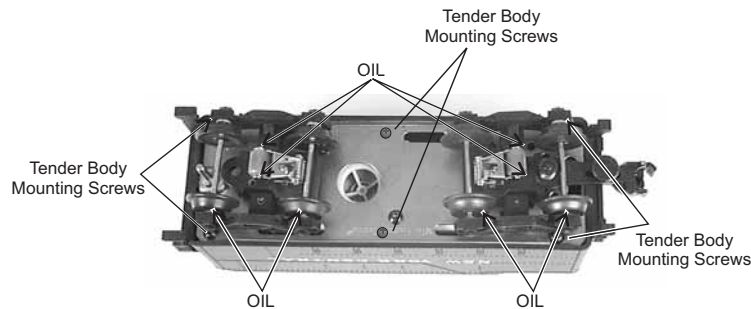
Figure 9: Lubricate The Tender Chassis Trucks
