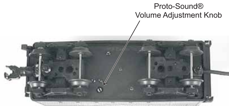
Figure 6: Adjusting The ProtoSound® Volume
