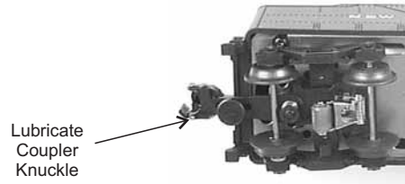
Figure 5: Lubricating The ProtoCouplers
