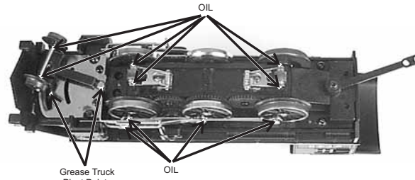
Figure 8: Lubricating The Locomotive Chassis
