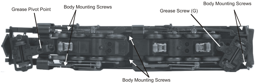
Figure 6. Removing the Body and Lubricating the Grease Points
