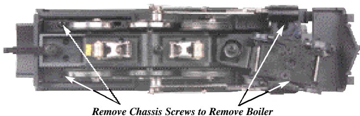
Figure 7 - Removing the Chassis
