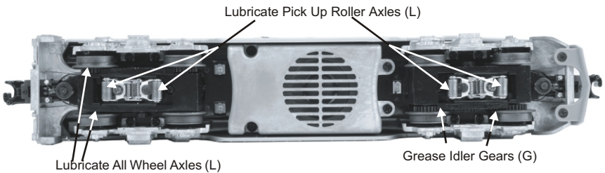
Figure 5: Lubrication Points
