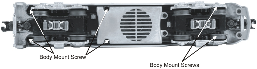
Figure 6: Mounting Screws
