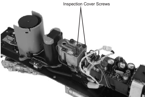
Figure 11: Inspecting the Smoke Unit Wick
