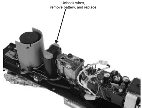
Figure 9: Replacing the Battery (Remove the remaining 2 screws on the fuel tank to access the battery).
