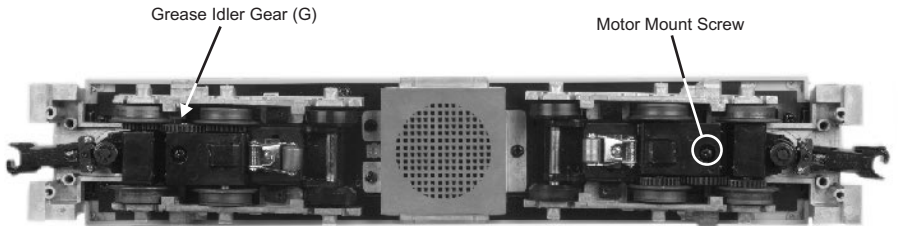
Figure 6: Locations of Greasing Points on the Locomotive
