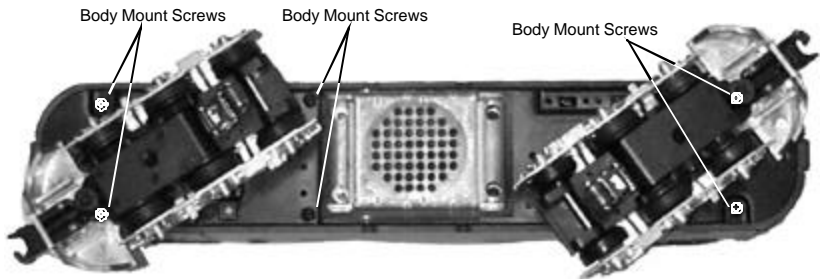
Figure 9: Removing the Body Mount Screws
