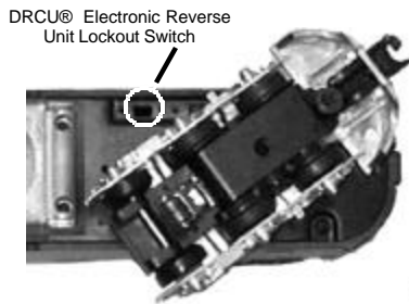
Figure 1: Proto sound® DCRU® Lockout Switch
