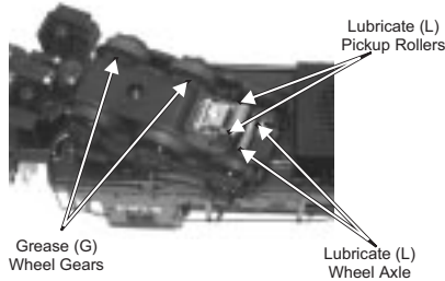
Figure 6: Lubricating The Locomotive Chassis
