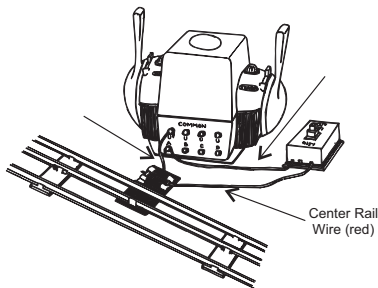
Figure 5: Wiring Up A Bell Button
