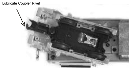
Figure 3: Lubricating The ProtoCouplers
