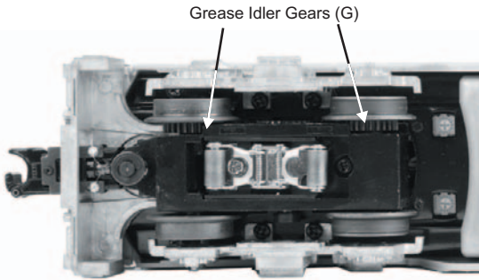
Figure 6. Greasing The Idler Gears
