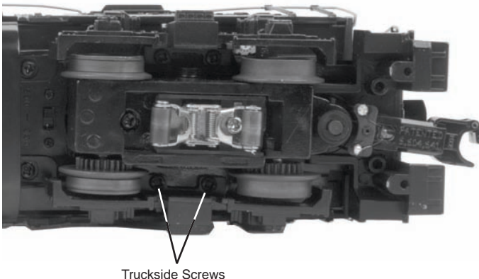
Figure 9: Truckside Screws
