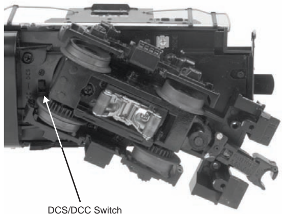
Figure 4: Changing from DCS to DCC Mode
