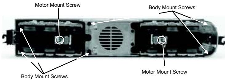
Figure 9: Body Removal Screw Locations and Motor Mounting Screws
