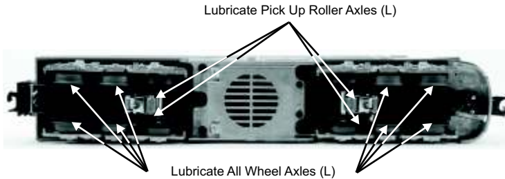
Figure 1: Lubrication Points on the Locomotive
