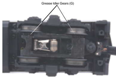
Figure 4: Greasing The Idler Gears
