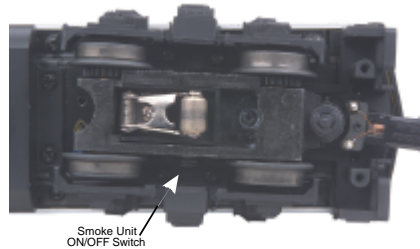
Figure 3. Smoke Unit ON/OFF Switch
