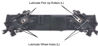
Figure 1. Lubrication Points on the Locomotive
