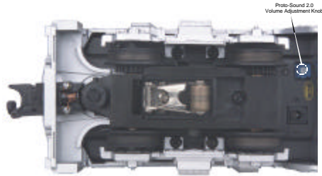
Figure 2: Manual Proto-Sound 2.0 Volume Adjustment
