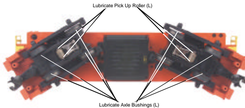
Figure 1. Lubrication Points on the Locomotive
