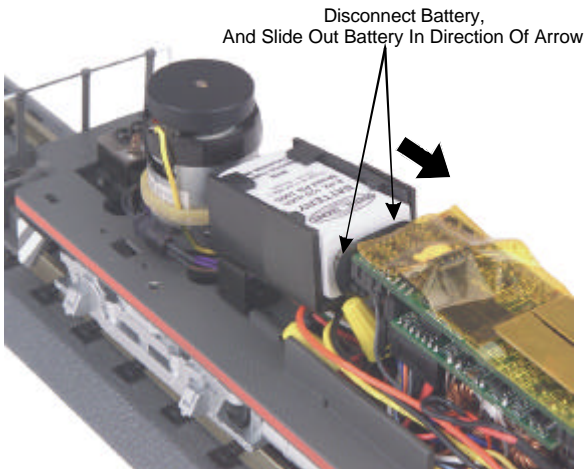
Figure 8: Removing The Battery
