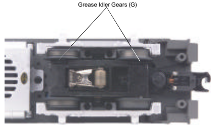
Figure 4: Greasing The Idler Gears
