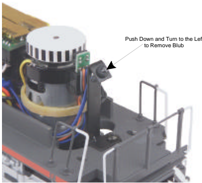
Figure 6: Removing The Replaceable Lights
