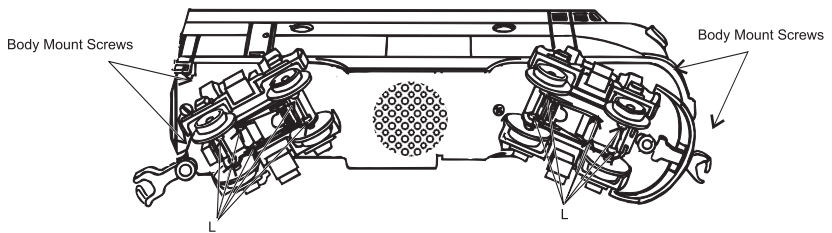
Figure 1: Lubricating The Chassis
