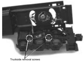
Figure 4. Screws to Remove to Access the Traction Tires
