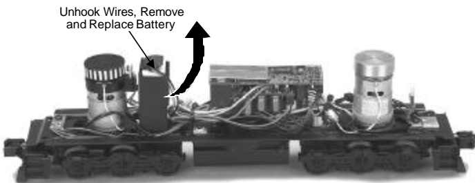
Figure 6. Removing and Replacing the Battery
