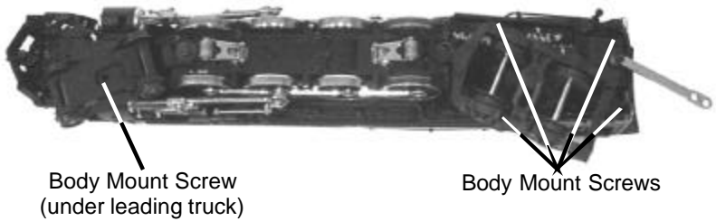
Figure 10: Removing The Boiler From The Chassis
