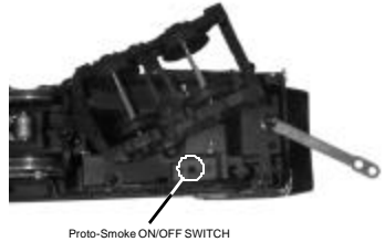
Figure 3: Smoke Unit Switch
