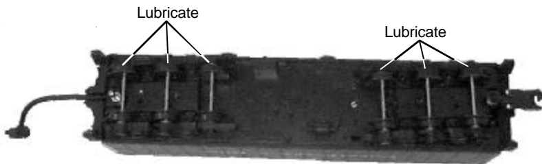
Figure 9: Lubricate The Tender Chassis Trucks
