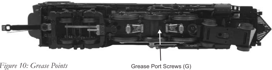
Figure 10: Grease Points
