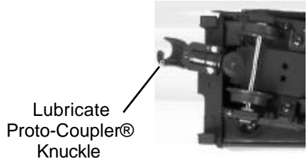
Figure 5: Lubricating The ProtoCoupler
