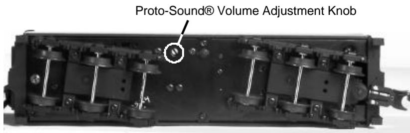
Figure 6: Adjusting The ProtoSound® Volume
