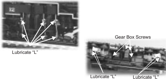
Figure 8: Lubricating The Locomotive Chassis
