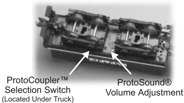
Figure 6: Adjusting The ProtoSound® Volume
