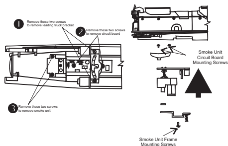
Figure 4: Inspecting The Smoke Unit
