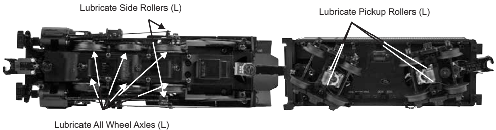
Fig. 1: Lubricating the Locomotive
