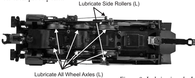
Figure 8: Lubricating the Locomotive
