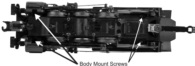
Figure 10: Removing the Body
