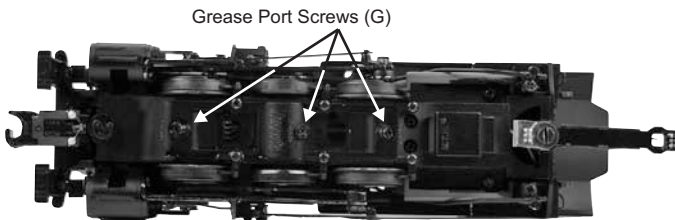
Figure 9: Grease Points
