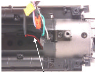
Wires for headlight
