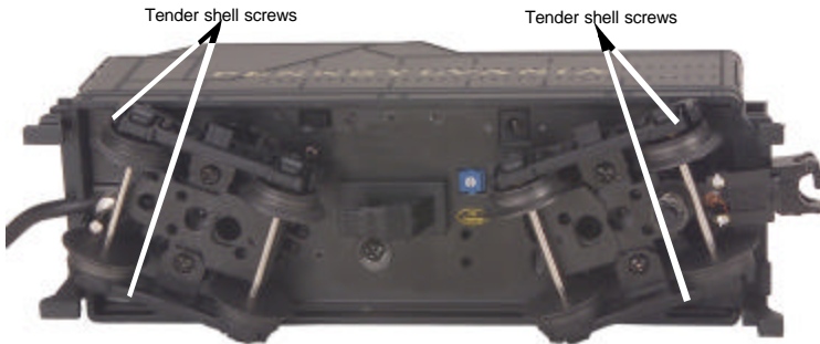
Figure 10: Removing The Tender Body
