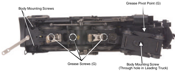
Figure 6: Removing The Body
