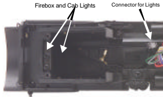
Figure 9: Boiler Connector Cables
