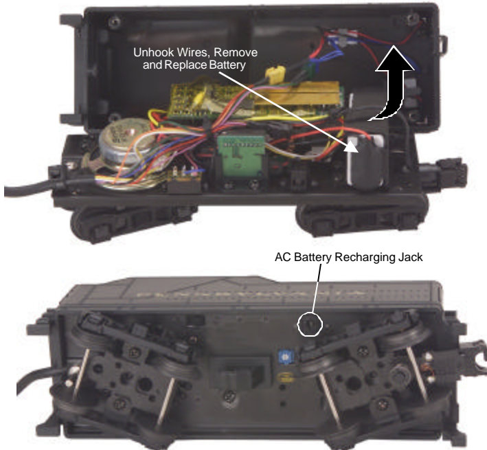
Figure 115: Replacing The Battery And Locating The Battery Recharging Jack
