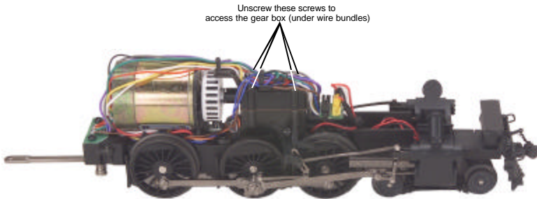
Figure 7: Opening The Gearbox
