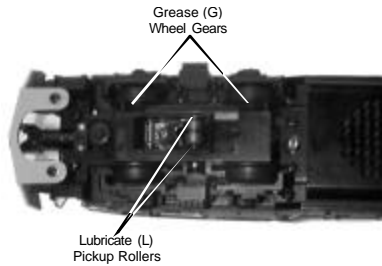
Figure 6: Lubricating The Locomotive Chassis
