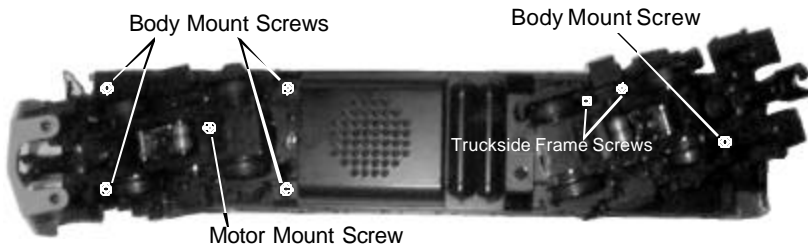
Figure 7: Lubricate The Tender Chassis Trucks
