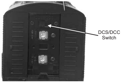
Figure 6: Changing from DCS to DCC Mode
