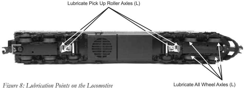
Figure 8: Lubrication Points on the Locomotive
