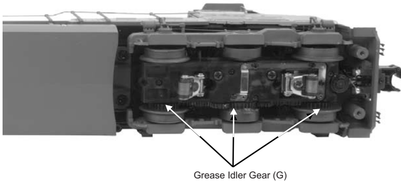
Figure 10: Greasing the Idler Gears
