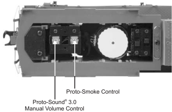
Figure 7: Manual Volume Control/Smoke Volume Control
