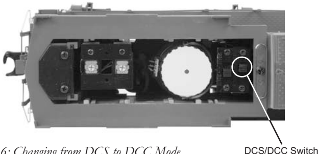
Figure 6: Changing from DCS to DCC Mode
