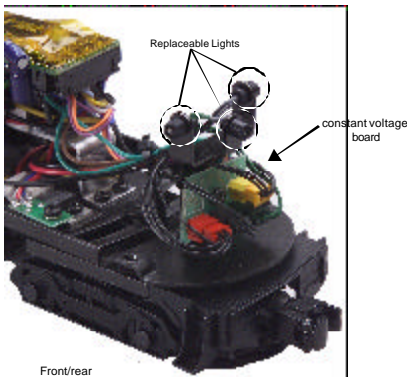
Figure 8. Locations of Replacable Lights
