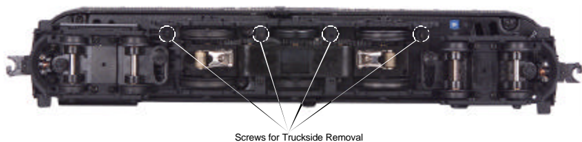
Figure 8. Locations of Truckside Mounting Screws
