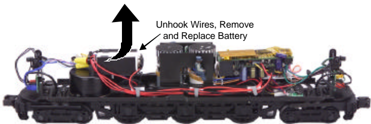
Figure 9. Replacing the Battery
