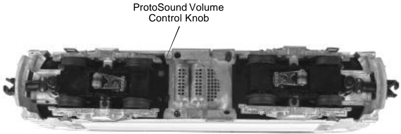
Figure 4: Adjusting The ProtoSound Volume
