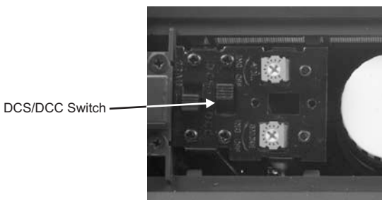
Figure 6: Changing from DCS to DCC Mode
