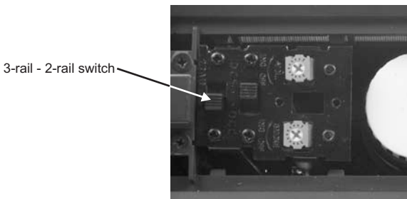
Figure 5: 3-Rail Pickups
