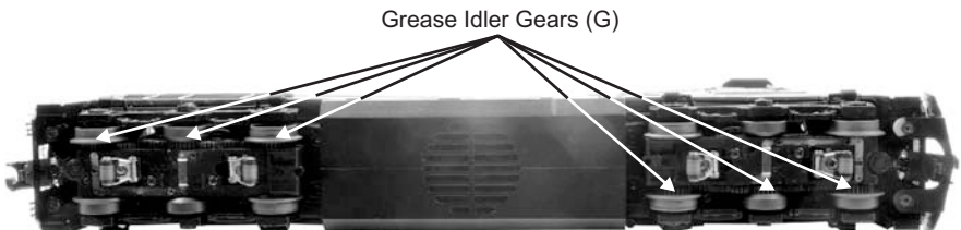
Figure 10: Greasing The Idler Gears
