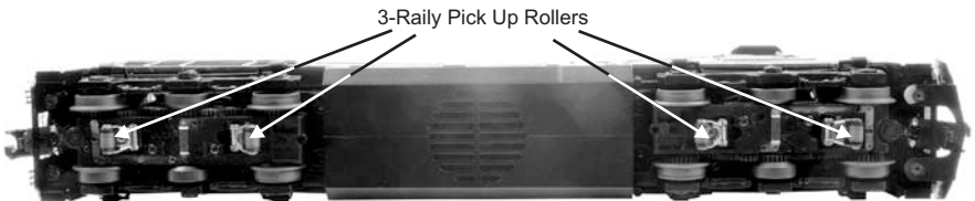
Figure 4: 3-Rail Pickups
