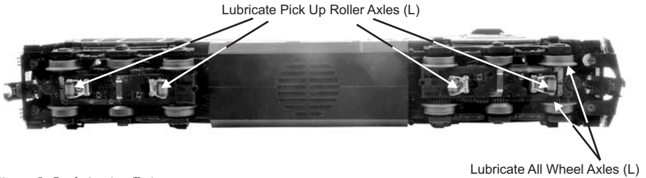
Figure 8: Lubrication Points
