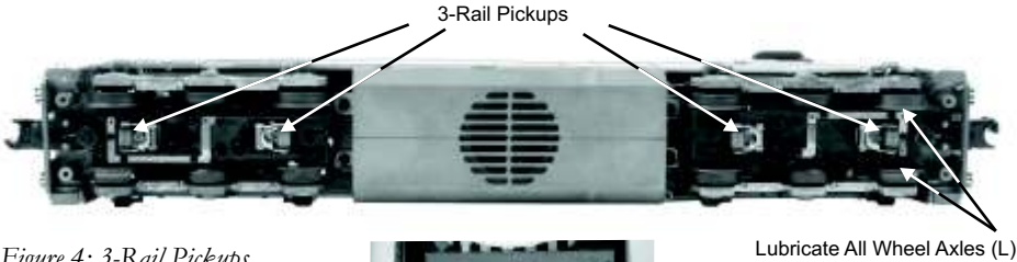
Figure 4: 3-Rail Pickups
