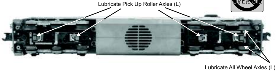
Figure 8: Lubrication Points
