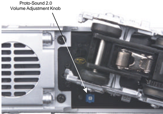
Figure 5: Proto-Sound Manual Volume Adjustment
