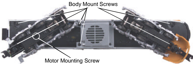
Figure 6: Removing the body from the chassis
