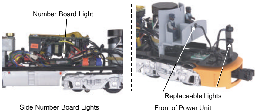
Figure 8: Replaceable light bulb locations
