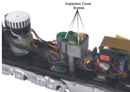
Figure 12: Inspecting The Smoke Unit Wick
