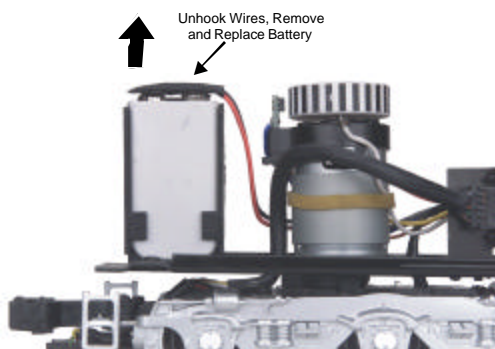
Figure 10: Removing the battery
