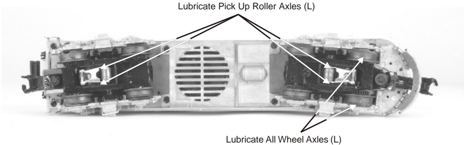
Figure 1. Lubrication Points on the Locomotive
