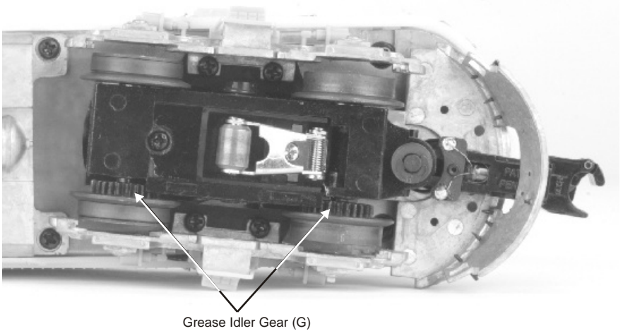
Figure 7. Greasing The Idler Gears
