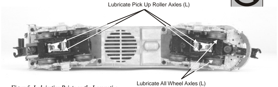
Figure 5. Lubrication Points on the Locomotive
