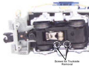
Figure 7. Locations of Truckside Mounting Screws
