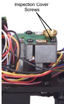
Figure 4. Inspecting the Smoke Unit
