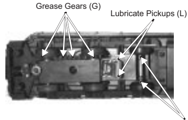
Figure 6: Lubricating The Locomotive Chassis
