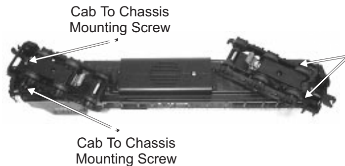
Figure 8: Removing The Body From The Chassis
