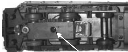
Truck Block/Motor Mount Attachment Screw
