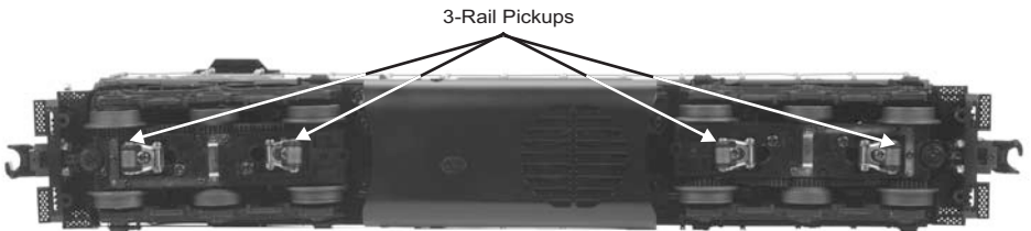
Figure 5: 2-Rail/3-Rail Operation
