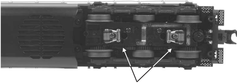
Figure 10: Greasing the Idler Gears Grease Idler Gear (G)
