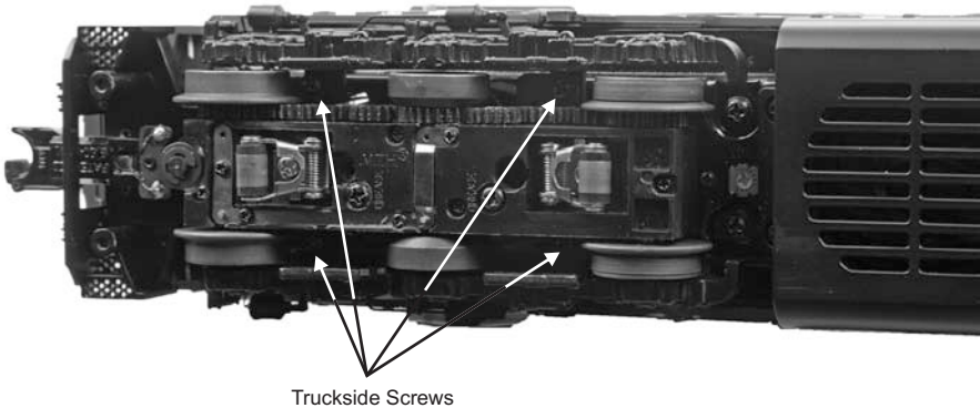
Figure 11: Truckside Screws
