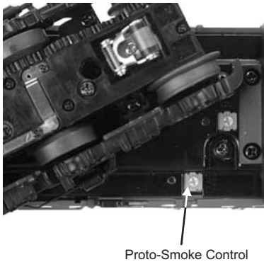
Figure 3: Accessing the Controls
