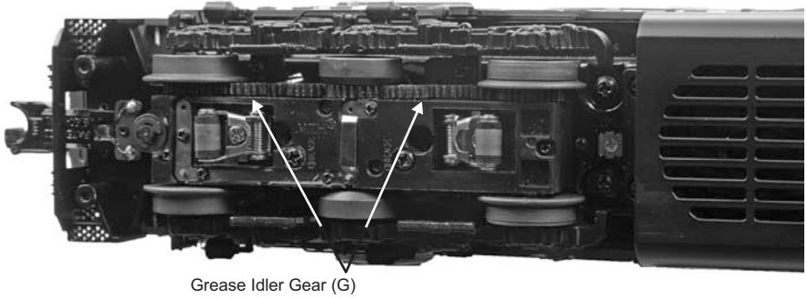
Figure 10: Greasing the Idler Gears
