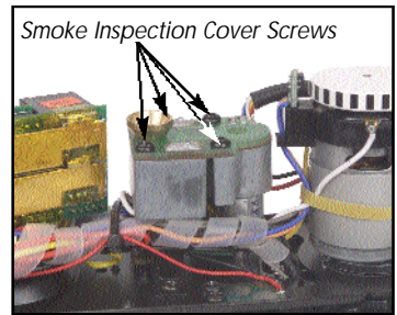
Figure 7 - Smoke Unit Inspection Cover
