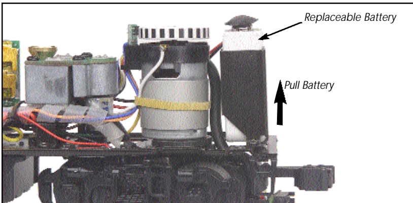
Figure 11- Replacing the Battery
