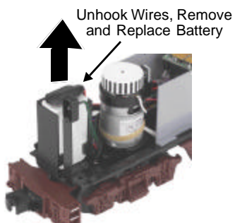
Figure 10: Removing the battery
