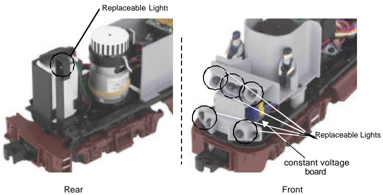
Figure 8: Replaceable light bulb locations
