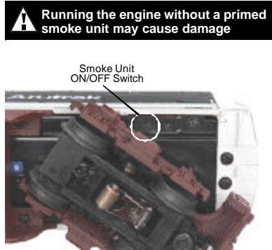
Figure 3: Smoke Unit Switch Location
