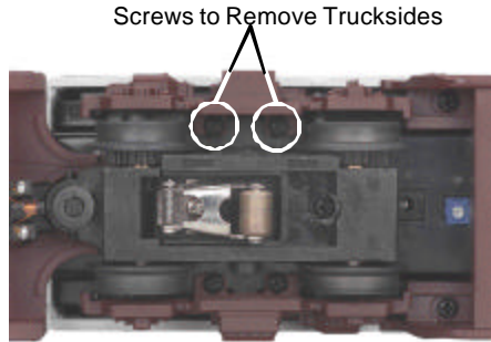
Figure 7: Removing the trucksides
