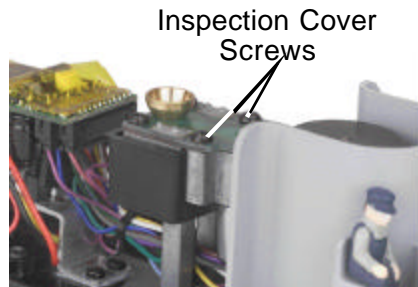
Figure 12: Inspecting The Smoke Unit Wick
