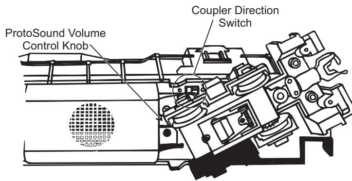
Figure 4: Adjusting The ProtoSound® Volume and selecting the ProtoCoupler
