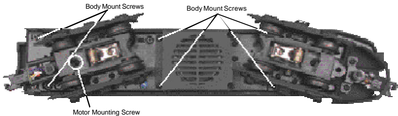
Figure 6: Body Mounting Screw Locations
