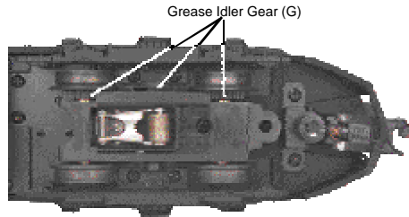
Figure 7: Power Truck Grease Locations
