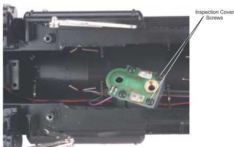
Figure 16: Inspecting The Smoke Unit Wick
